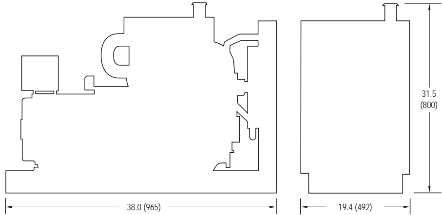
NL753W2 Overall Dimensions L x W x H: 38.0 x 19.4 x 31.5 inch (965 x 492 x 800 mm)
